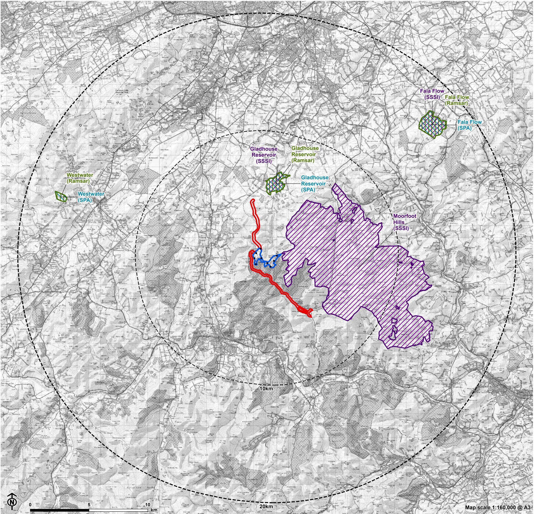
Figure 8.2: Site Location in Relation to Statutory Designated Sites of Ornithological Interest
