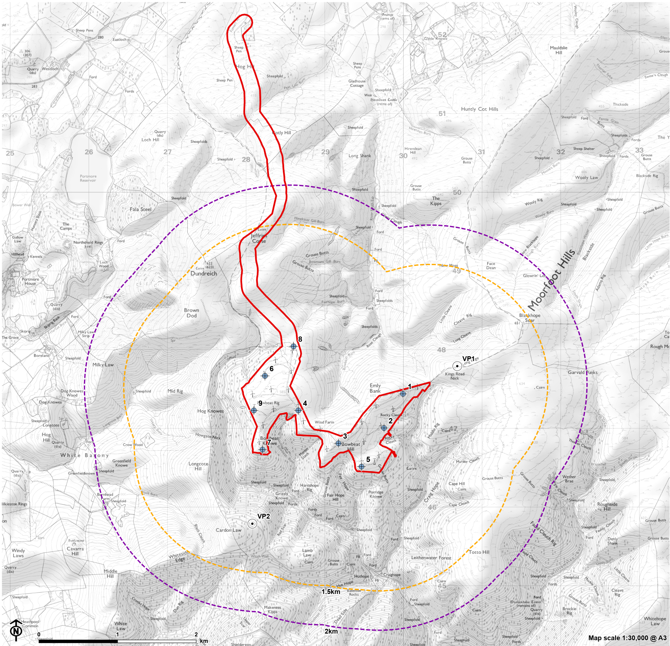
Figure 8.1: Ornithology Survey Areas
